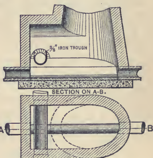
FIG. 5. CROSSING MANHOLE.
